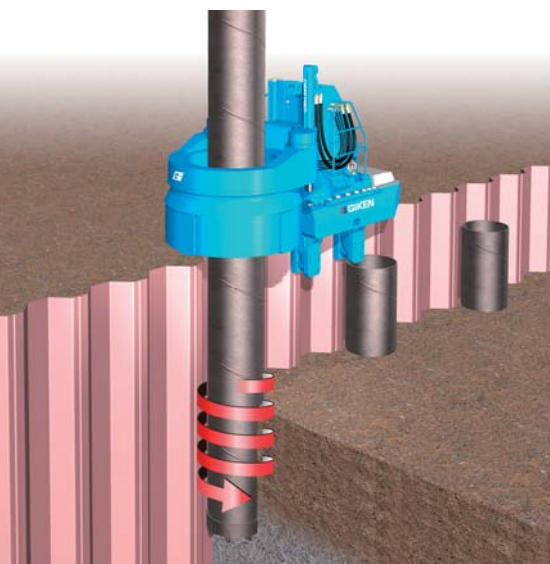
Combi-Gyro Wall
