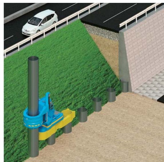
Backfill Retaining Wall Type
