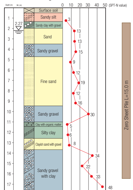
▼ Borehole Log
